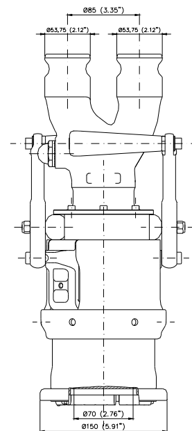
Femalecoupling
