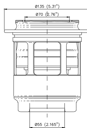
Female coupling
